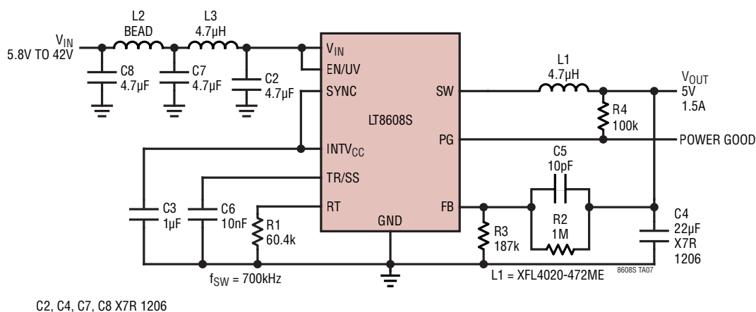
Ultralow EMI 5V 1.5A Step-Down Converter
