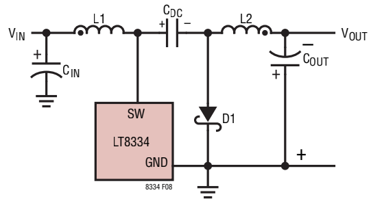
Figure 8. A Simplified Inverting Converter
