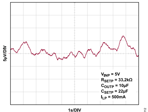
Figure 112. Positive Output Noise: 0.1 Hz to 10 Hz ( C_{SETP} = 22\mu F )
