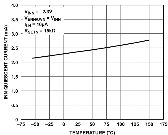
Figure 23. INN Quiescent Current vs. Temperature ( V_{ENN/UVN} = V_{INN} )
