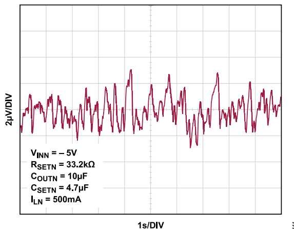
Figure 111. Negative Output Noise: 0.1 Hz to 10 Hz (C_SETN = 4.7 μF)
