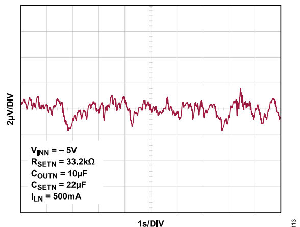
Figure 113. Negative Output Noise: 0.1 Hz to 10 Hz ( C_{SETN} = 22\mu F )
