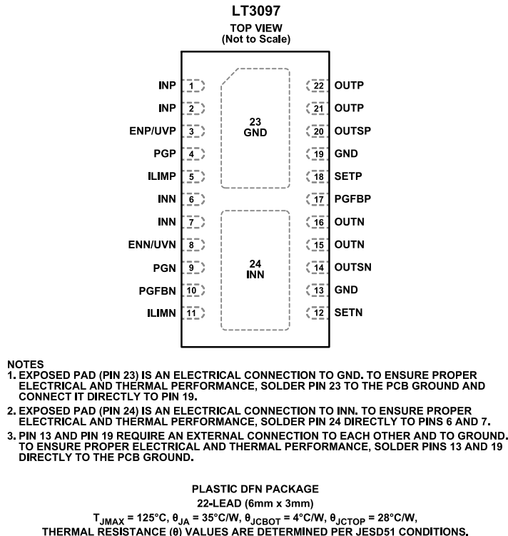
Figure 3. Pin Configuration
