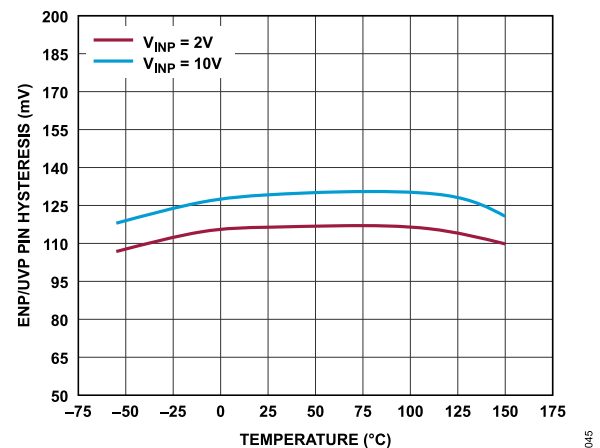
Figure 45. ENP/UVP Pin Hysteresis vs. Temperature
