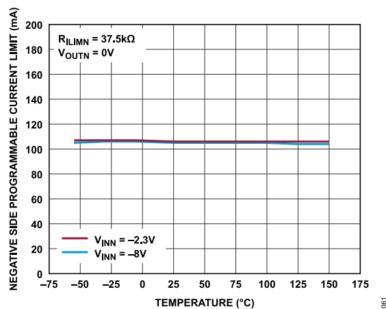
Figure 61. Negative Side Programmable Current Limit vs. Temperature (100 mA)
