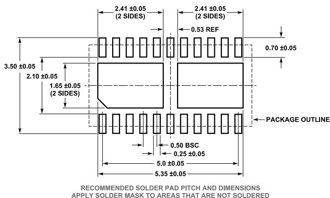
Figure 132. 22-Lead, 6 mm x 3 mm, Plastic DFN (05-08-7071) Dimensions shown in millimeters
