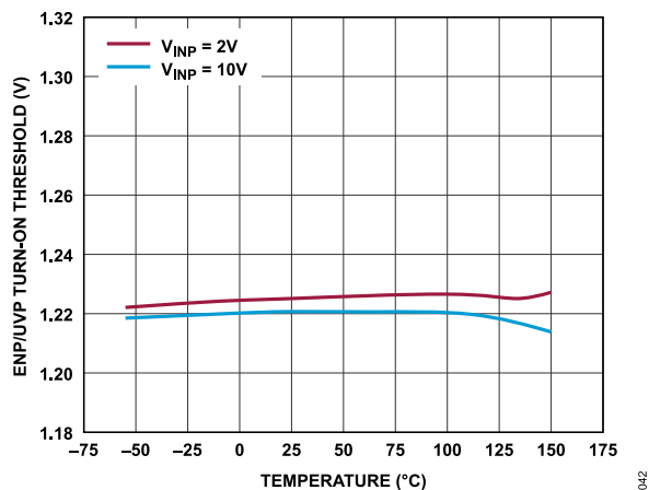
Figure 42. ENP/UVP Turn-On Threshold vs. Temperature
