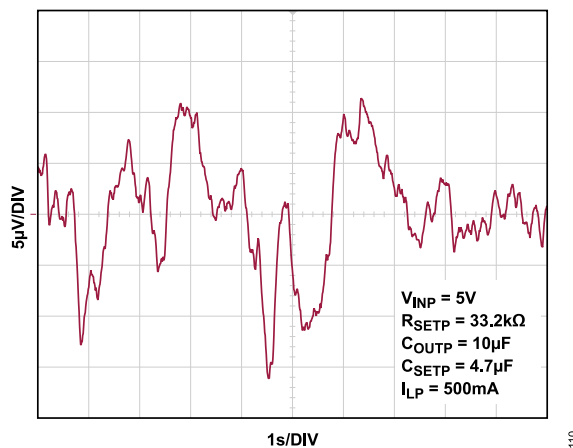
Figure 110. Positive Output Noise: 0.1 Hz to 10 Hz (C_SETP = 4.7 μF)
