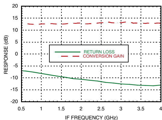
IF Bandwidth [1]
