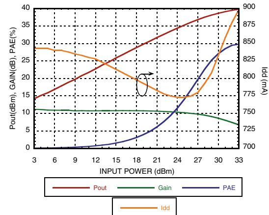
Power Compression @ 3 GHz
