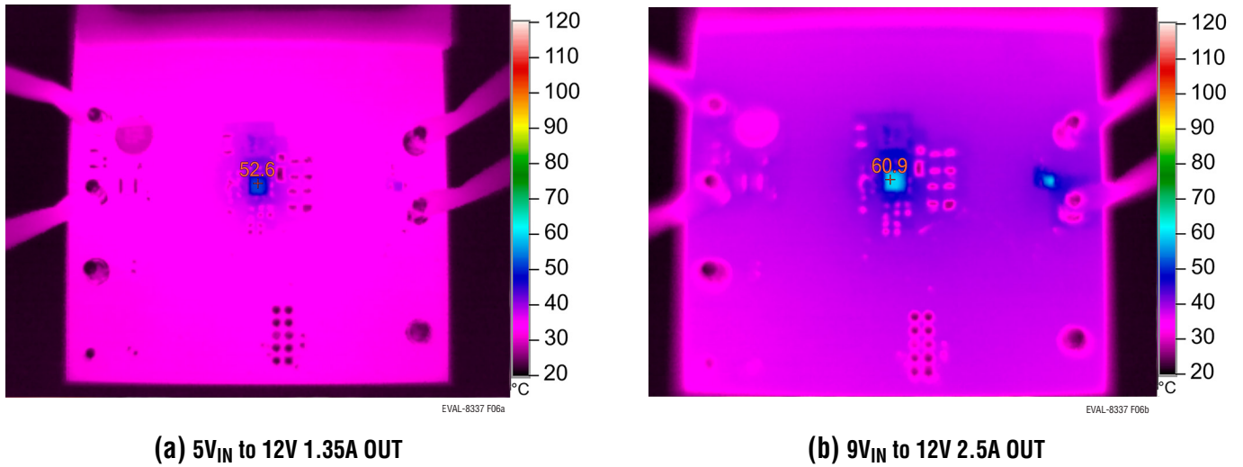
Figure 6. EVAL-LT8337-1-AZ Thermals
