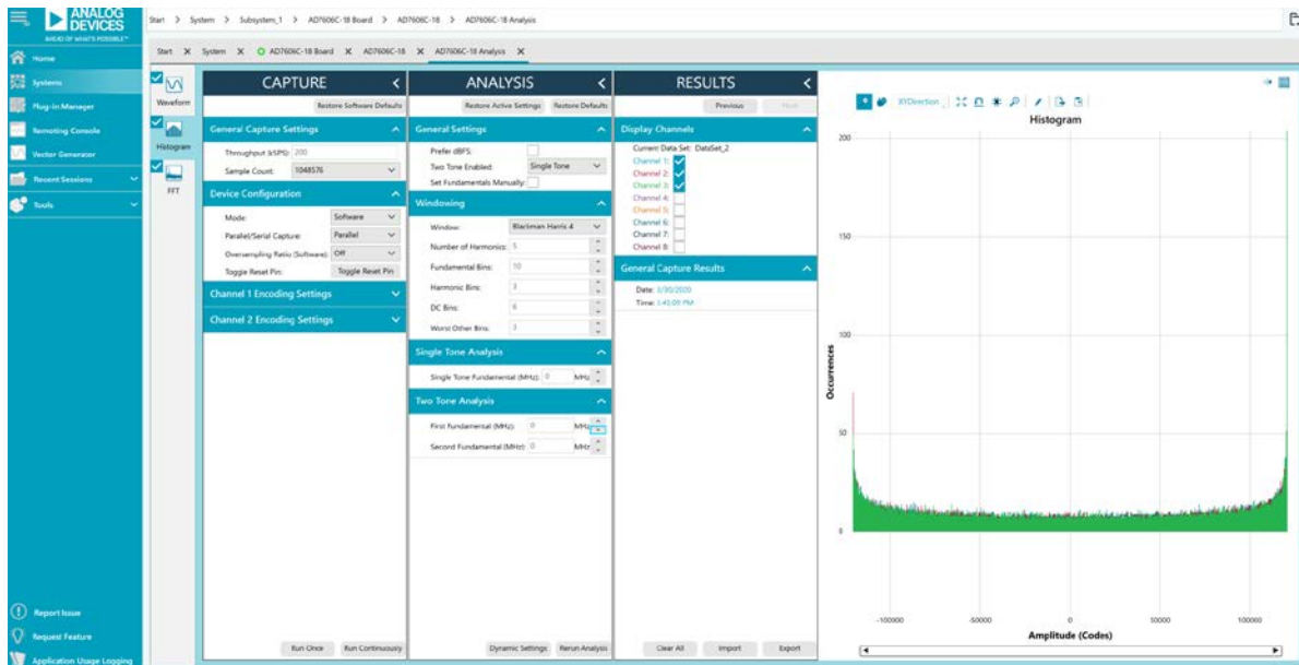
Figure 17. Histogram Tab
