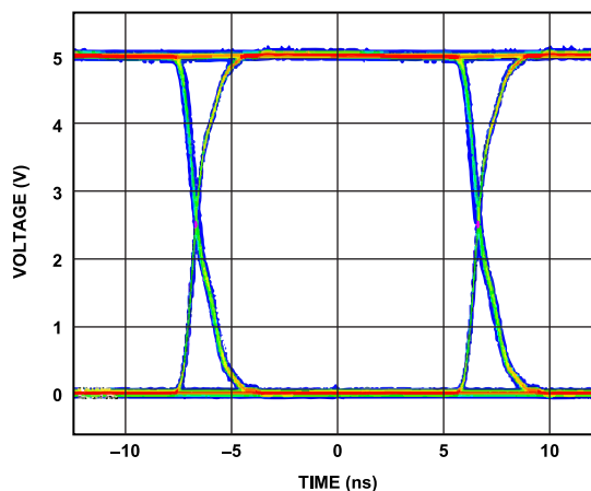
Figure 22. ADuM220N/ADuM221N/ADuM225N/ADuM226N Eye Diagram
