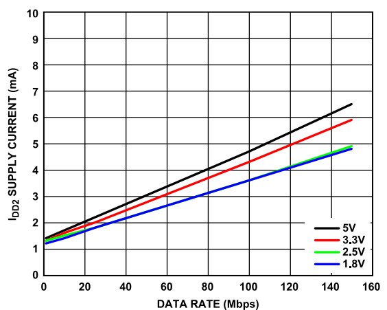
Figure 12. ADuM220N/ADuM225N I_{DD2} Supply Current vs. Data Rate at Various Voltages
