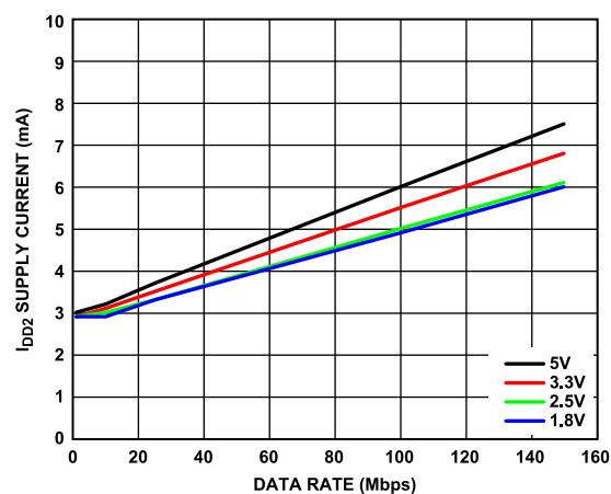
Figure 15. ADuM221N/ADuM226N I_{DD2} Supply Current vs. Data Rate at Various Voltages
