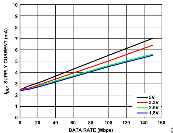
Figure 14. ADuM221N/ADuM226N I_{DD1} Supply Current vs. Data Rate at Various Voltages
