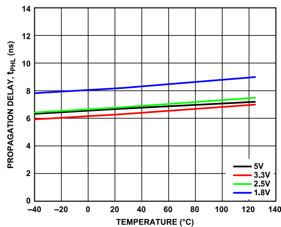
Figure 16. Propagation Delay for Logic Low Output ( t_{PHL} ) vs. Temperature at Various Voltages
