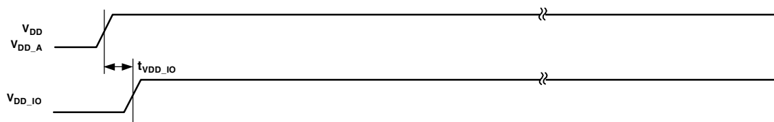
Figure 12. Power-Up Timing
