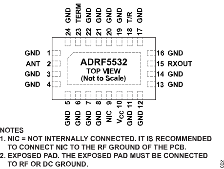
Figure 2. Pin Configuration
