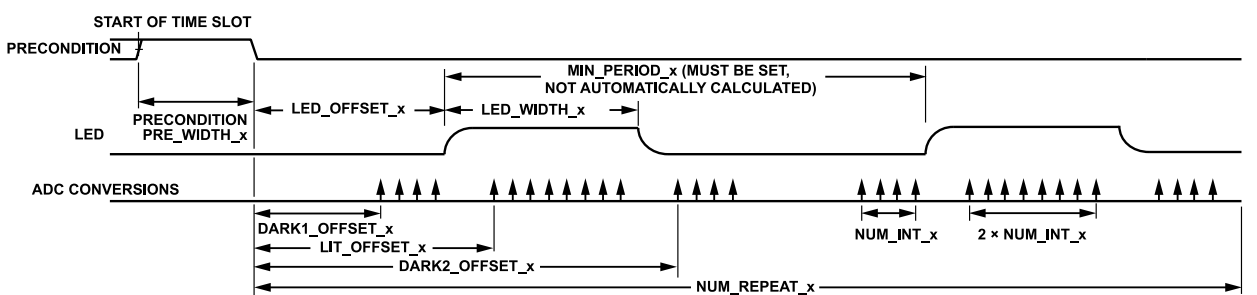
Figure 35. Two-Region Digital Integration Mode Timing Diagram
