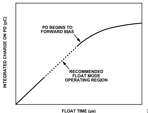
Figure 28. Integrated Charge on the Photodiode vs. Float Time
