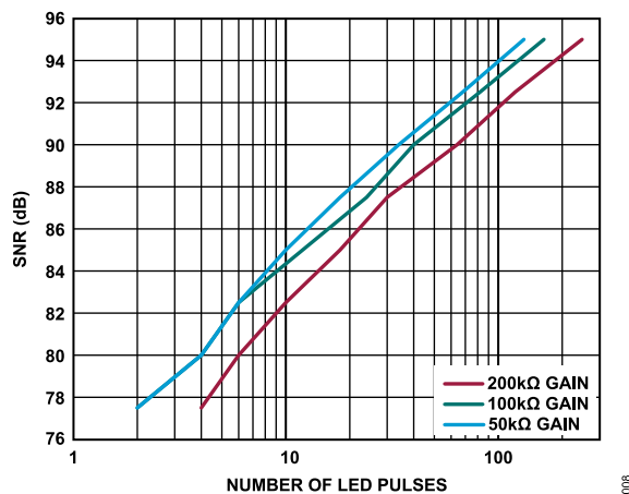
Figure 8. SNR vs. Number of Pulses, C_{PD} = 70 pF
