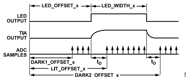
Figure 36. Proper Placement of ADC Sampling Edges in Digital Integration Mode
