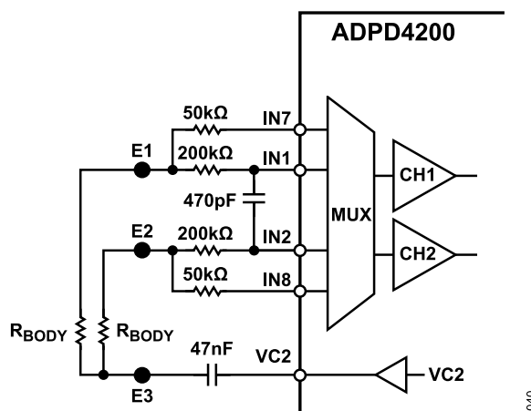
Figure 40. Circuit Used for Lead Off Detection Measurement
