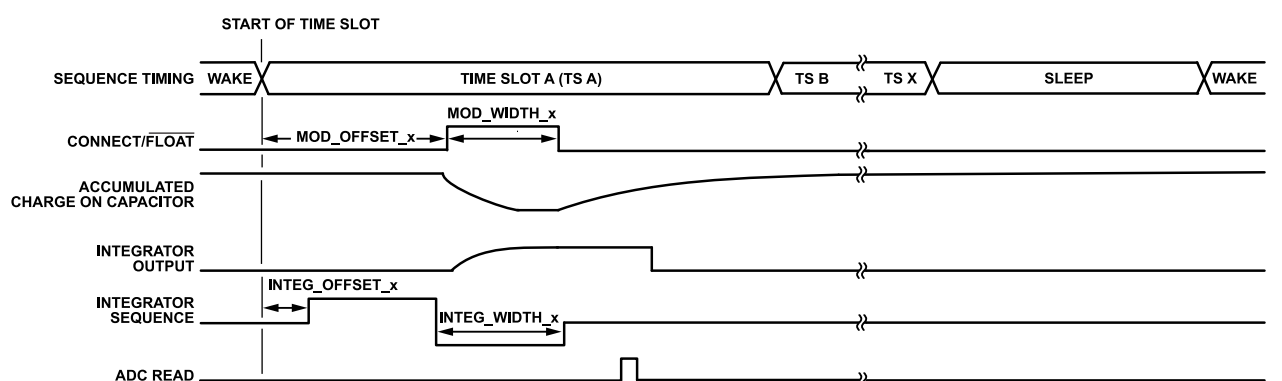
Figure 39. Sleep Float Mode Timing Diagram
