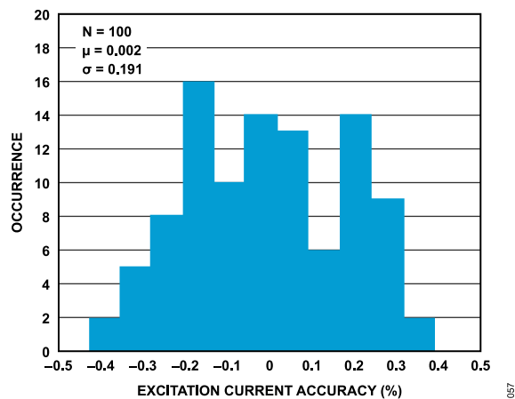
Figure 57. Excitation Current Initial Accuracy Histogram (100 \mu A)
