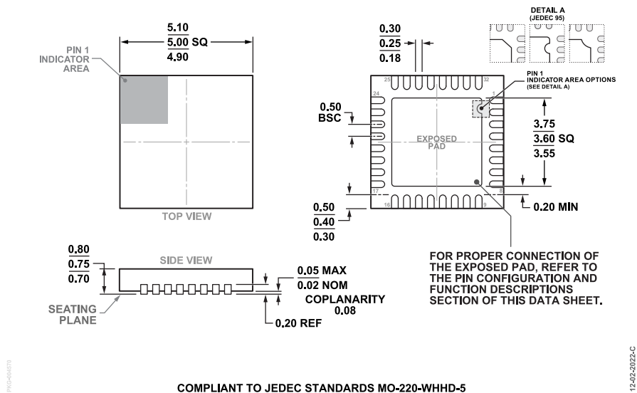
Figure 127. 32-Lead Lead Frame Chip-Scale Package [LFCSP] 5 mm x 5 mm Body and 0.75 mm Package Height (CP-32-12) Dimensions Shown in millimeters
