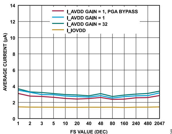
Figure 48. Duty-Cycling Current Consumption ( AV_{DD} and IOV_{DD} ), DUTY\_CYC\_RATIO = 1/16
