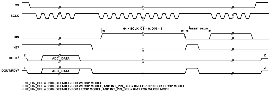
Figure 75. Software Reset Timing Diagram
