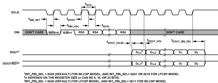
Figure 3. Read Cycle Timing Diagram, 3-Wire Mode (CSB_EN Bit Set to 0), \overline{\text{CS}} Pin Connected Low
