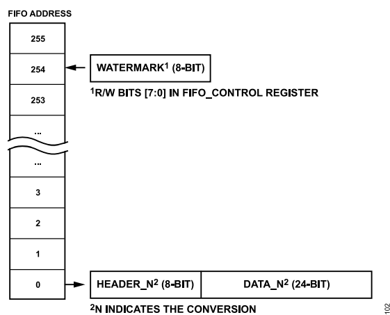
Figure 102. FIFO Structure
