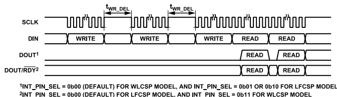
Figure 4. Delay Between Consecutive Serial Operations, 3-Wire Mode (CSB_EN Bit Set to 0), \overline{\text{CS}} Pin Connected Low
