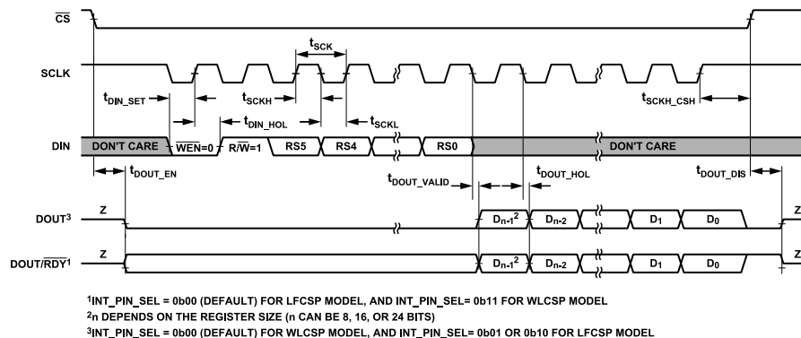
Figure 6. 3-Wire Mode Read Cycle Timing Diagram, 3-Wire Mode (CSB_EN Bit Set to 0), \overline{\text{CS}} Pin Used to Tristate the DOUT Pin
