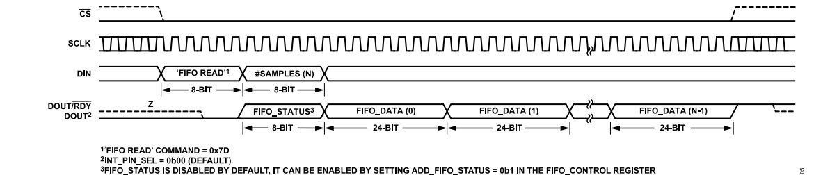
Figure 105. FIFO Readback (FIFO_STATUS Append On and FIFO_HEADER Append Off)
