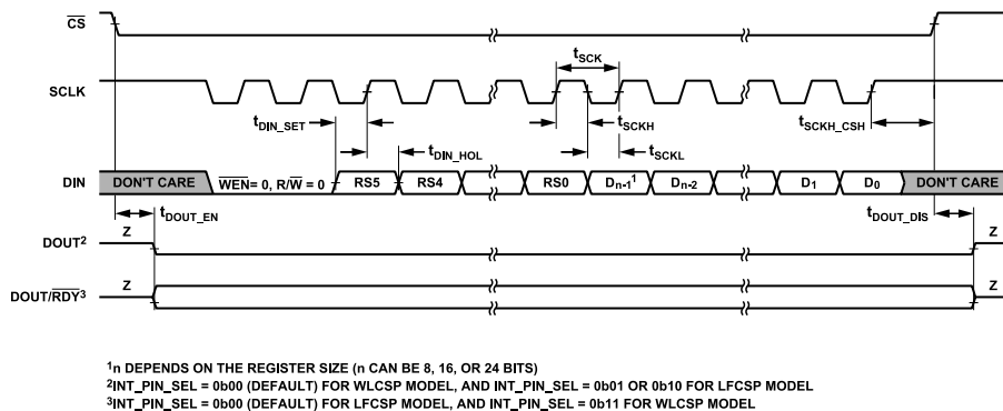
Figure 5. Write Cycle Timing Diagram, 3-Wire Mode (CSB_EN Bit Set to 0), \overline{\text{CS}} Pin Used to Tristate the DOUT Pin
