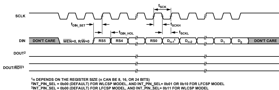
Figure 2. Write Cycle Timing Diagram, 3-Wire Mode ( \text{CS\_EN} Bit Set to 0), \overline{\text{CS}} Pin Connected Low
