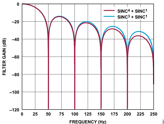
Figure 91. \text{Sinc}^3 + \text{Sinc}^1 and \text{Sinc}^4 + \text{Sinc}^1 Filter Response (FS = 6)
