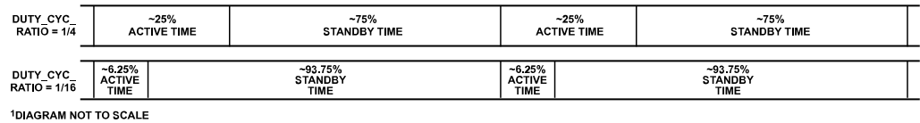
Figure 78. Duty Cycling Mode Diagram
