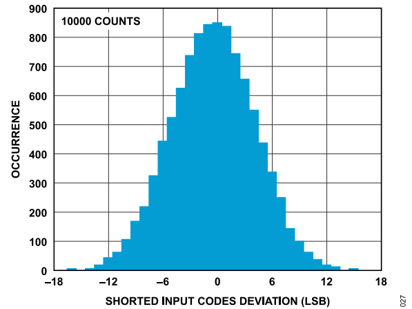
Figure 30. Noise Histogram Plot ( \text{Sinc}^4 Filter, ODR = 240 SPS, Gain = 1, Internal 1.25 V Reference)
