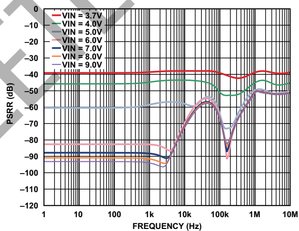
Figure 8. VOUT2 PSRR, I_{\text{OUT2}} = 50\ \text{mA}
