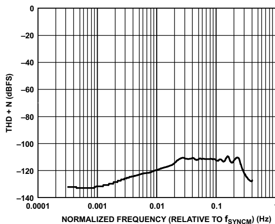
Figure 18. PDM Total Harmonic Distortion + Noise (THD + N) vs. Normalized Frequency (Relative to f_{\text{SYNC}} ), f_{\text{SYNC}} = 48 \text{ kHz}
