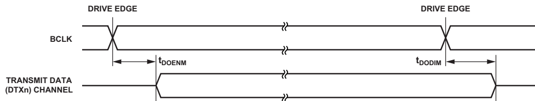
Figure 13. I²S Slave (A²B Main Node) Enable and Three-State Timing
