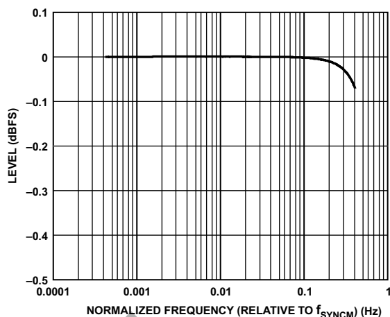
Figure 16. PDM Frequency Response, f_{\text{SYNC}} = 48 \text{ kHz}
