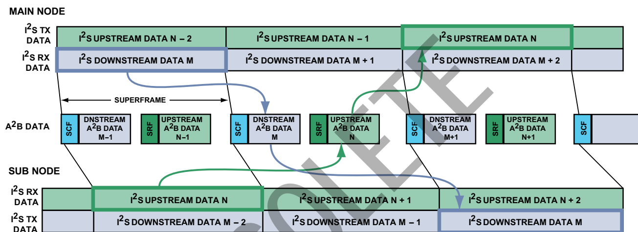
Figure 4. A²B Bus Synchronous Data Exchange
