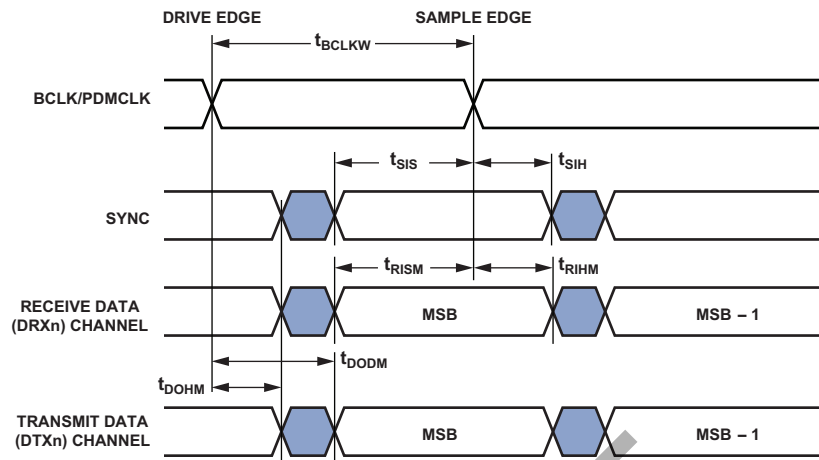
Figure 11. I²S Slave (A²B Main Node) Timing
