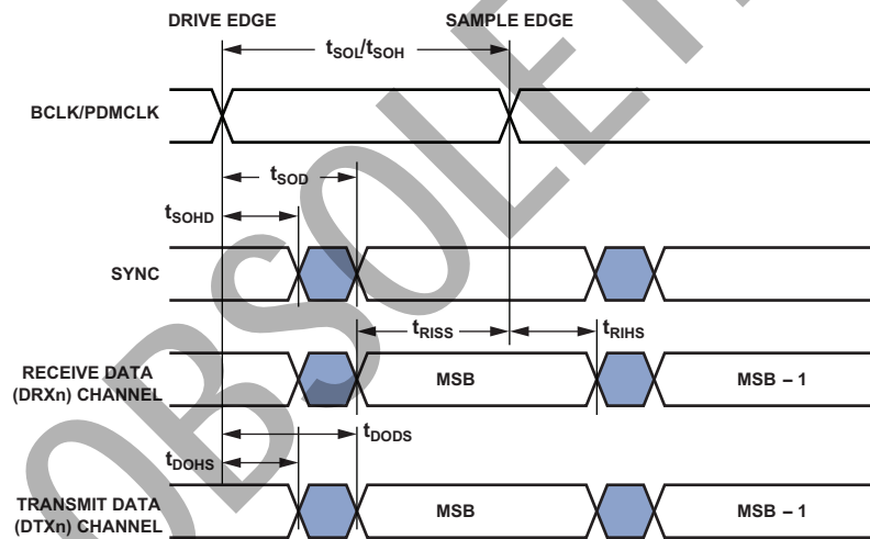
Figure 12. I²S Master (A²B Subordinate Node) Timing
