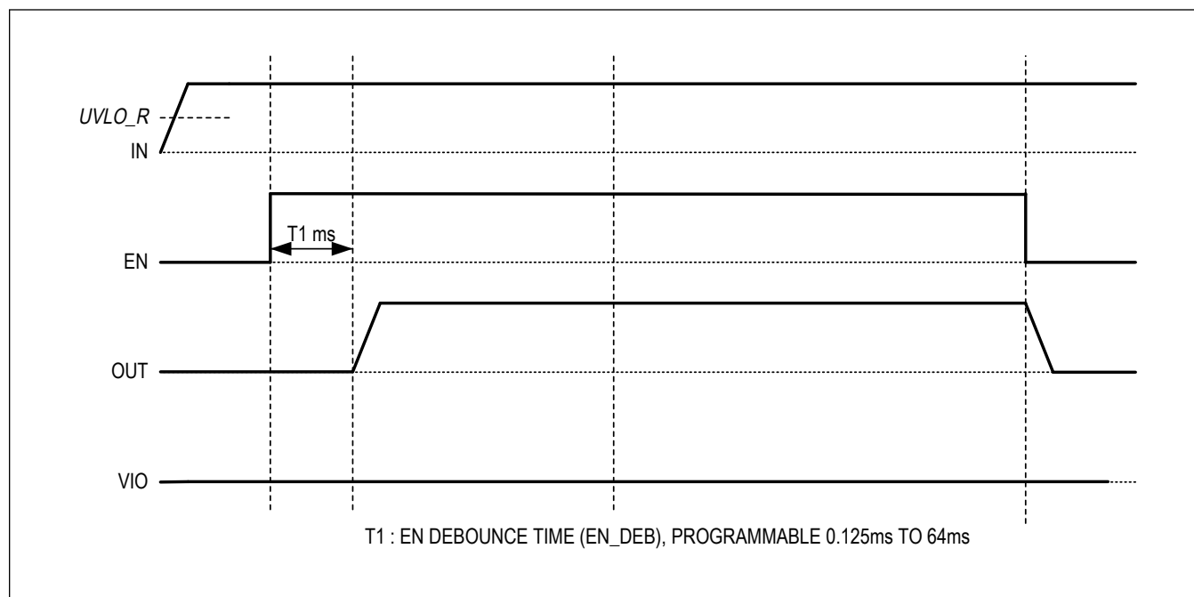
Figure 1. Enable Timing Waveform Without VIO
