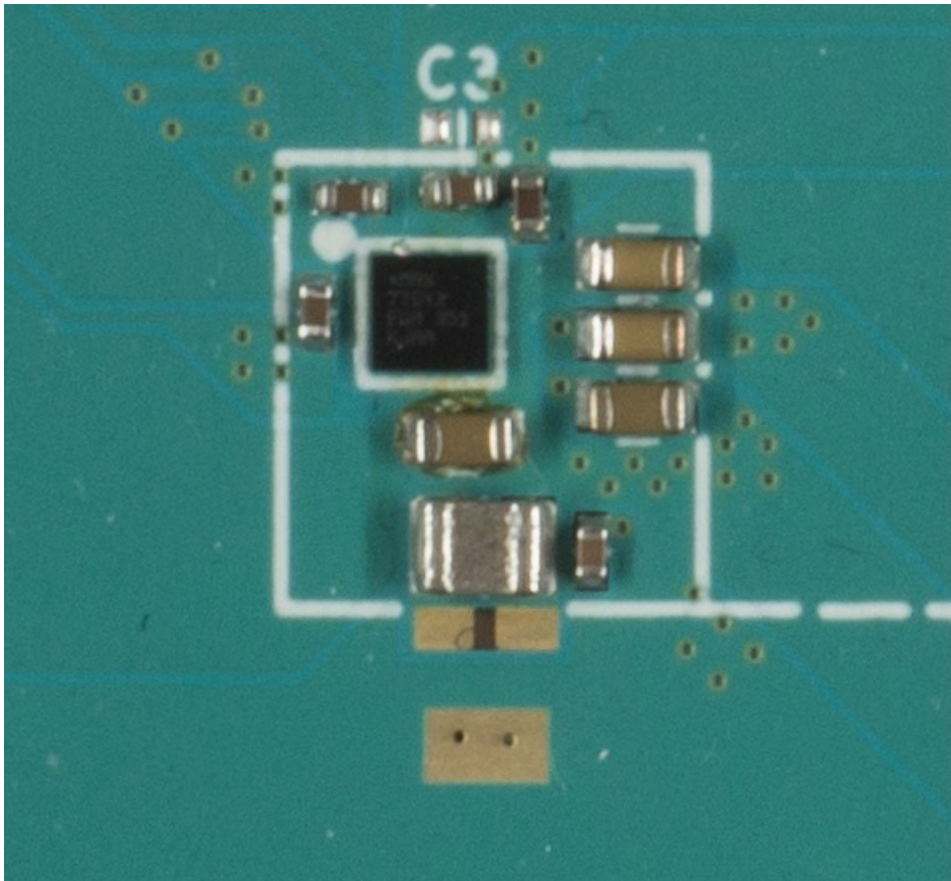
Figure 5. MAX77643 EV Kit Solution Area
