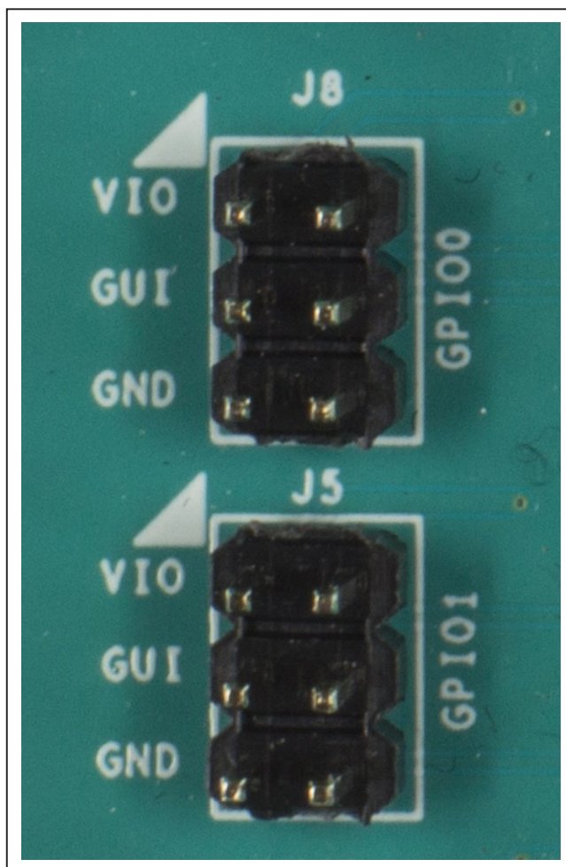
Figure 6. GPIO Headers
