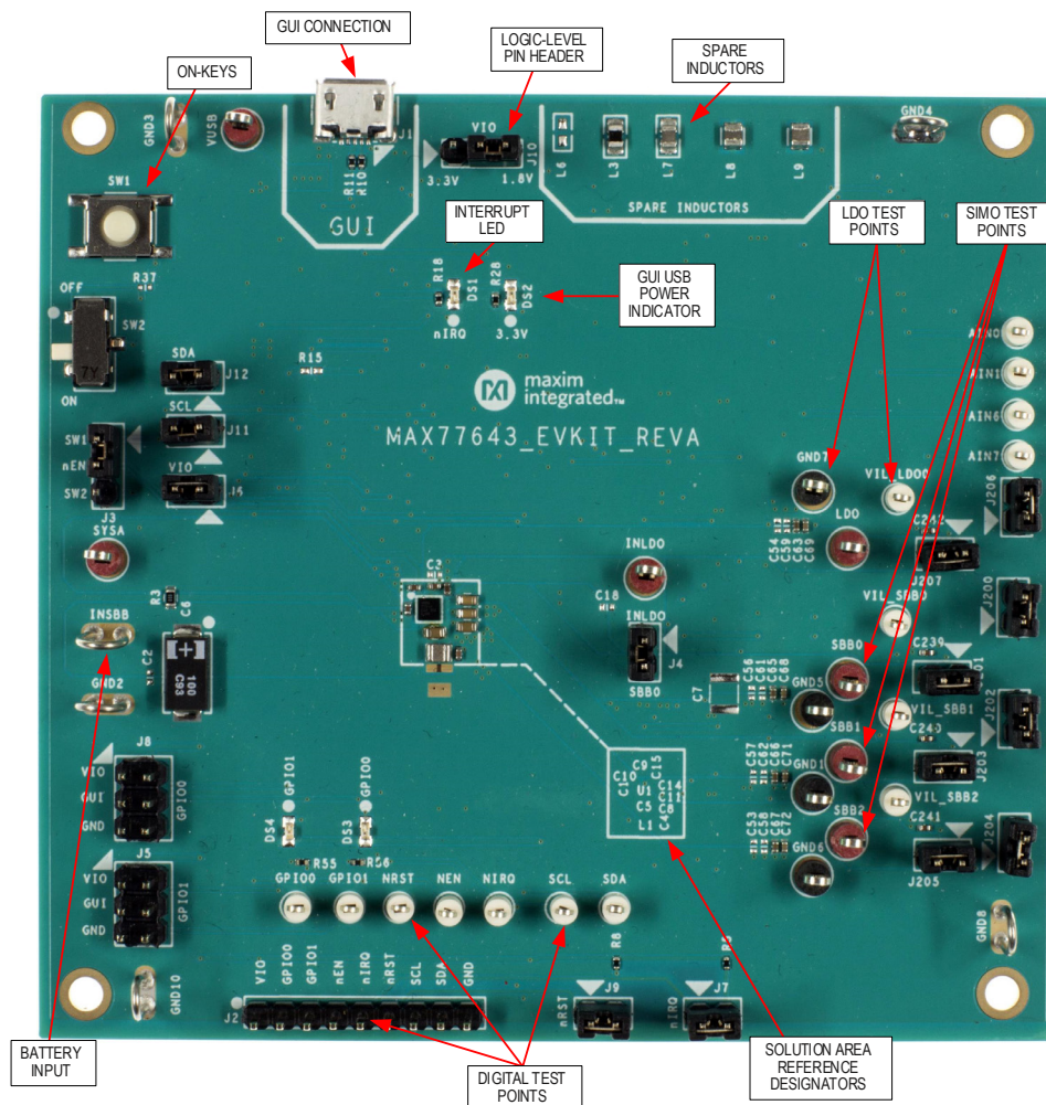
Figure 3. MAX77643 EV Kit Top View
