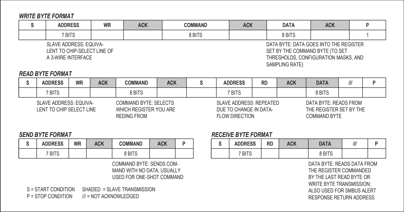
Figure 1. SMBus Protocols
