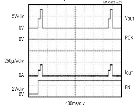
STARTUP WITH MIDSPAN MODE (DCA = V_{DIG} , INVALID PD (33k \Omega ))
