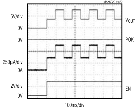
STARTUP WITH INVALID PD (15k \Omega )
