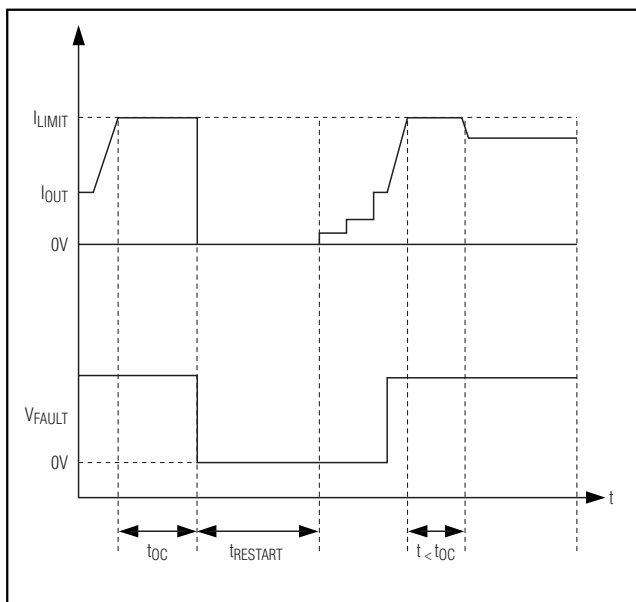
Figure 9. Overcurrent Response
