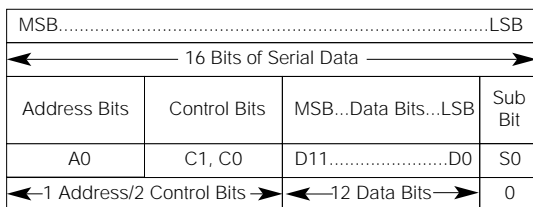
Figure 4. Serial-Data Format
