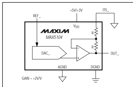
Figure 9. Unipolar Output Circuit (Rail-to-Rail)
