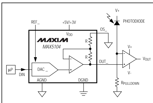
Figure 13. Digital Calibration
