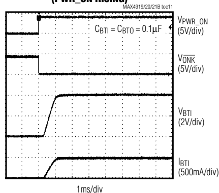
BATTERY-SWITCH TURN-ON RESPONSE (PWR_ON RISING)
