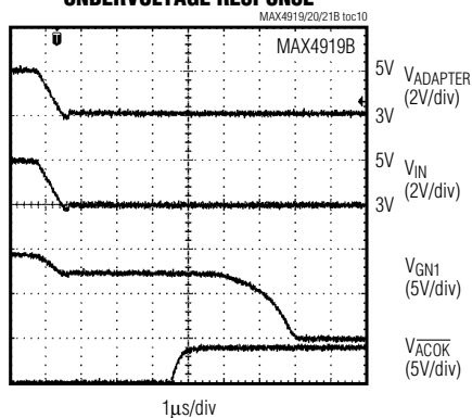
UNDERVOLTAGE RESPONSE
