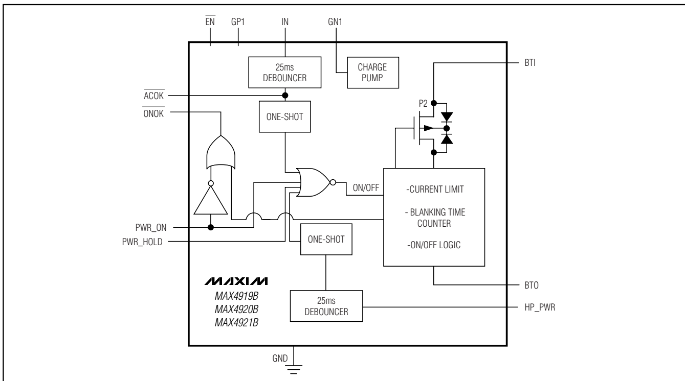
Figure 4. Functional Diagram
