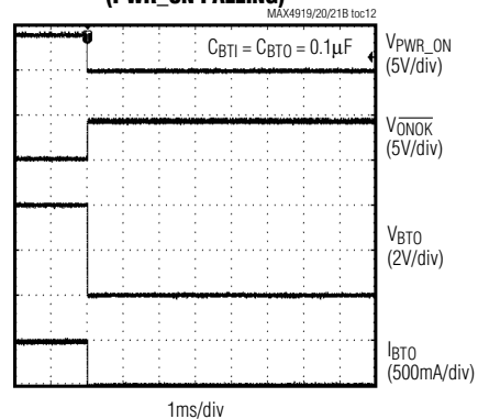
BATTERY-SWITCH TURN-OFF RESPONSE (PWR_ON FALLING)
