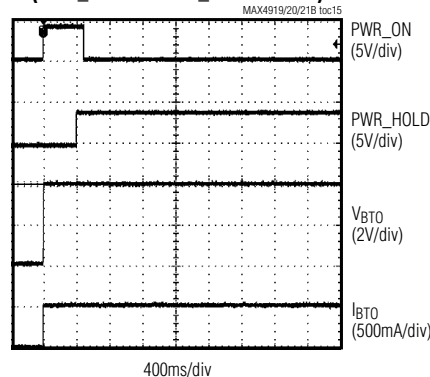
BATTERY SWITCH TURN-ON RESPONSE (PWR_ON AND PWR_HOLD RISING)
