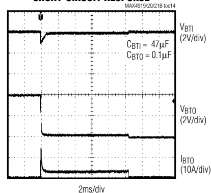
SHORT-CIRCUIT RESPONSE
