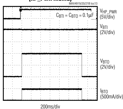
BATTERY-SWITCH TURN-ON RESPONSE (HP_PWR RISING)
