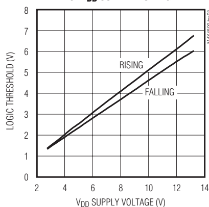
LOGIC THRESHOLD vs. V_{DD} SUPPLY VOLTAGE
