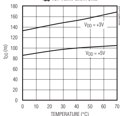
t_{D0} vs. TEMPERATURE
