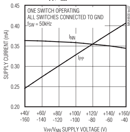
SUPPLY CURRENT vs. V_{PP}/V_{NN} SUPPLY VOLTAGE
