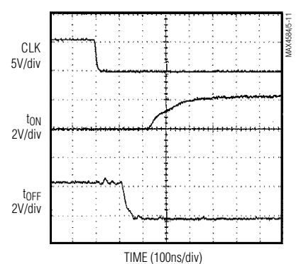
TURN-ON/TURN-OFF TIMES
