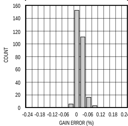
MAX4199 HISTOGRAM (GAIN ACCURACY BASED ON 280 UNITS)
