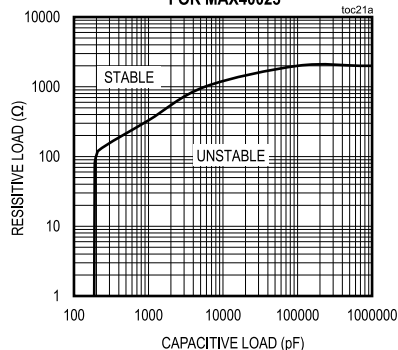
STABILITY vs. CAPACITIVE LOAD AND ISOLATION RESISTOR FOR MAX40023
