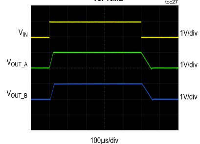
LARGE SIGNAL STEP RESPONSE vs. TIME
