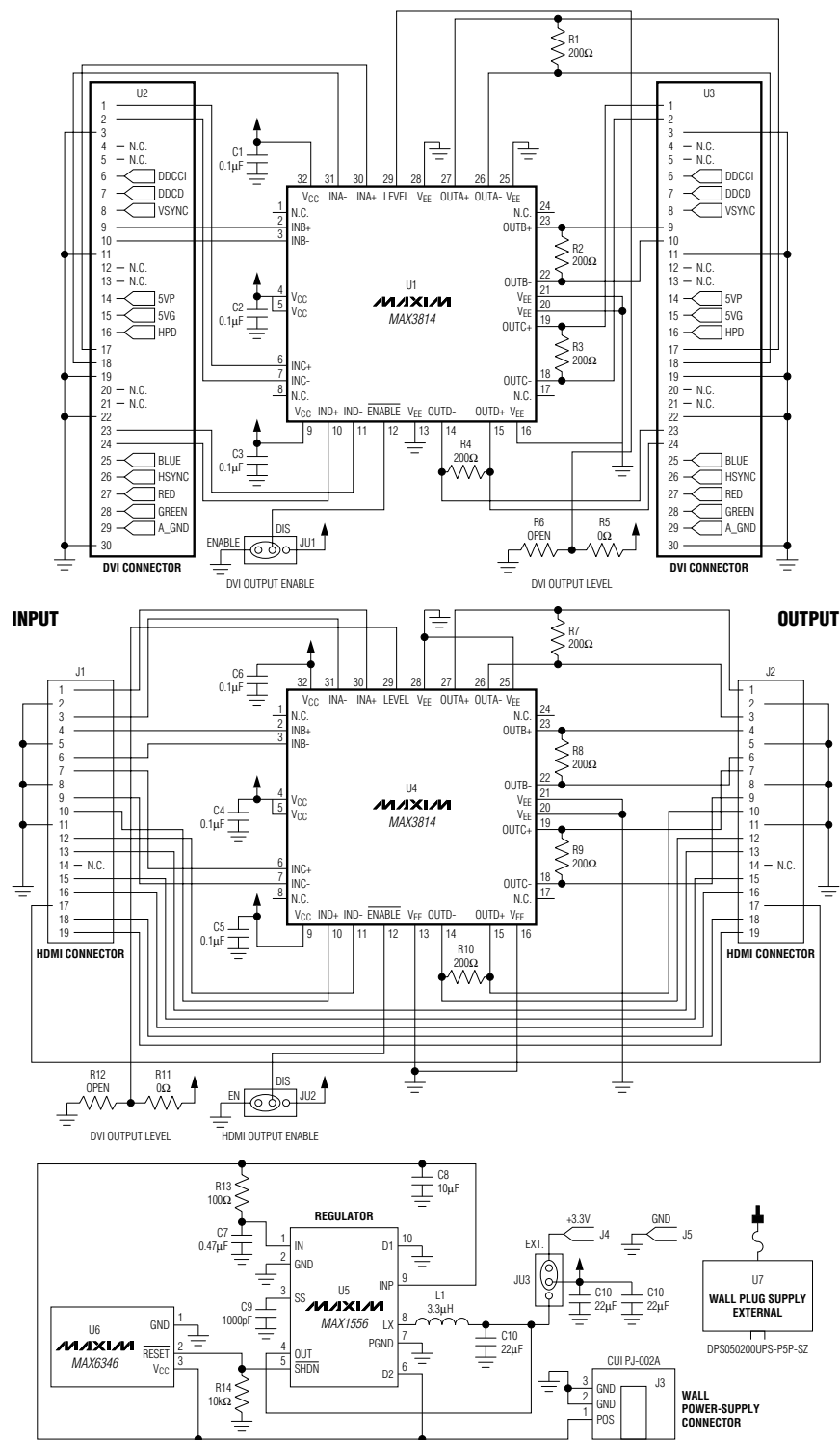
Figure 1. MAX3814 Customer Board Electrical Schematic
