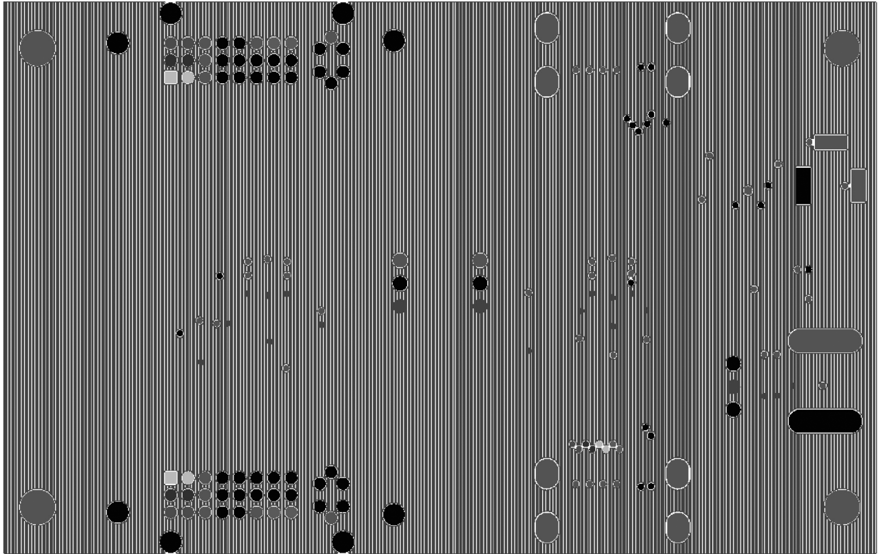
Figure 6. MAX3814 Evaluation Kit Power Plane
