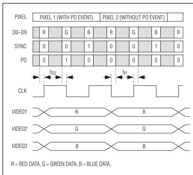
Figure 20. Configuration 1: Video Data Format
