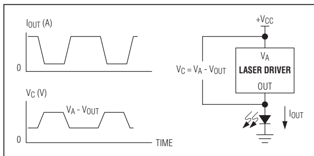
Figure 9. Output Compliance Voltage
