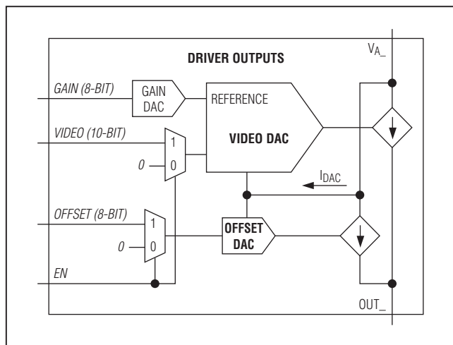
Figure 8. Driver Output
