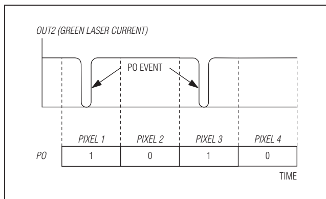
Figure 12. Periodic Off (PO) Example
