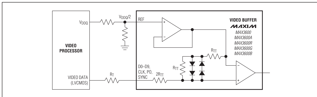
Figure 6. Video Inputs
