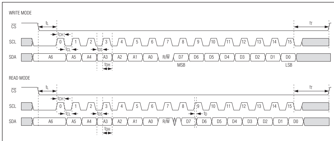
Figure 14. Serial Port Timing Diagram
