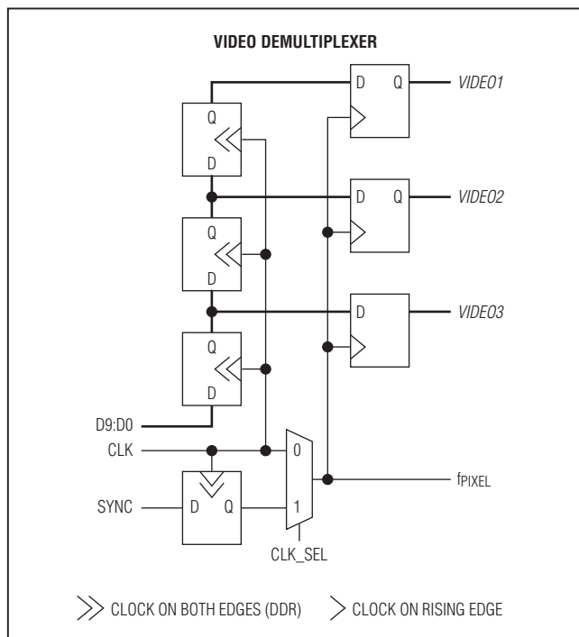
Figure 7. Video Demultiplexer
