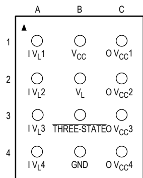
12 UCSP (1.5mm x 2.0mm) BOTTOM VIEW
