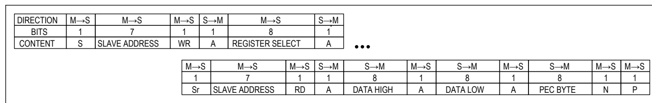
Figure 6. 2-Byte Read from MAX31827 with PEC Byte.
