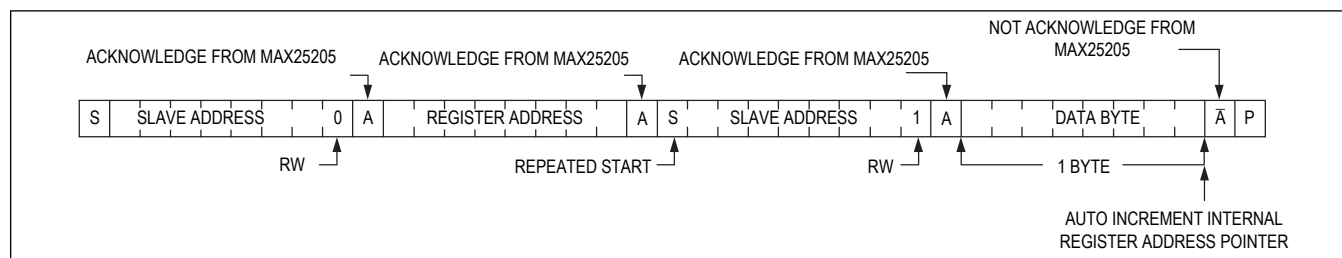
Figure 8. Reading 1 Byte of Indexed Data
