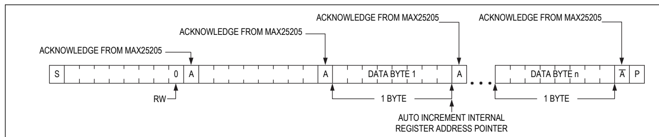
Figure 7. Write n Bytes
