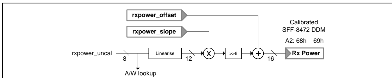
Figure 20. Calculating the Rx Power DDM
