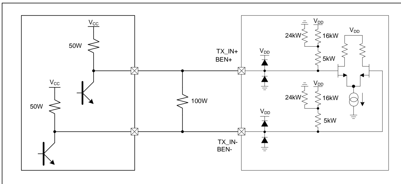
Figure 29. CML External Terminations
