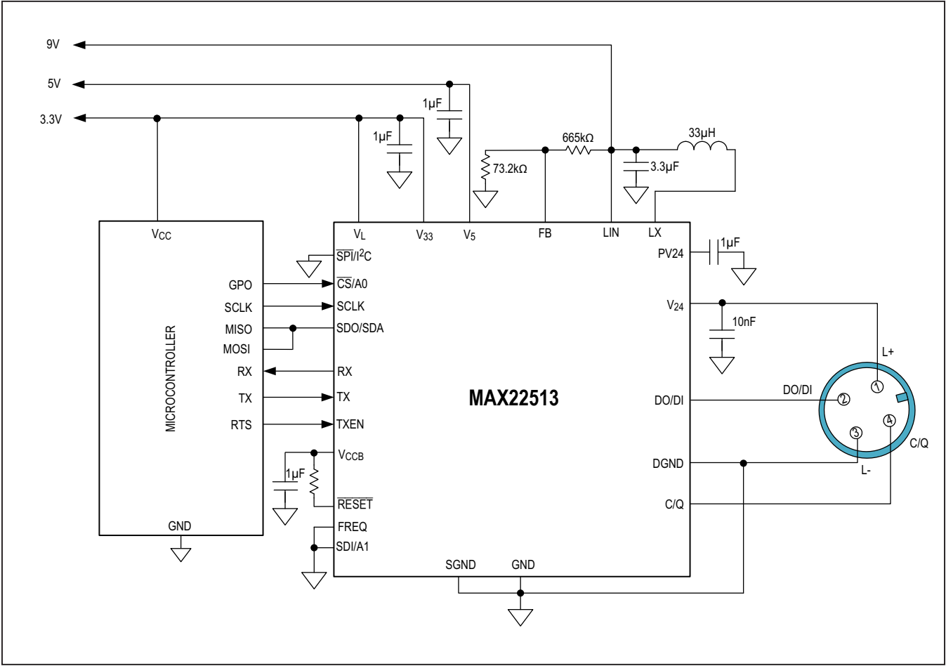
Half-Duplex SPI Interface Application with 9V/150mA DC-DC Output (12V, min Input)
