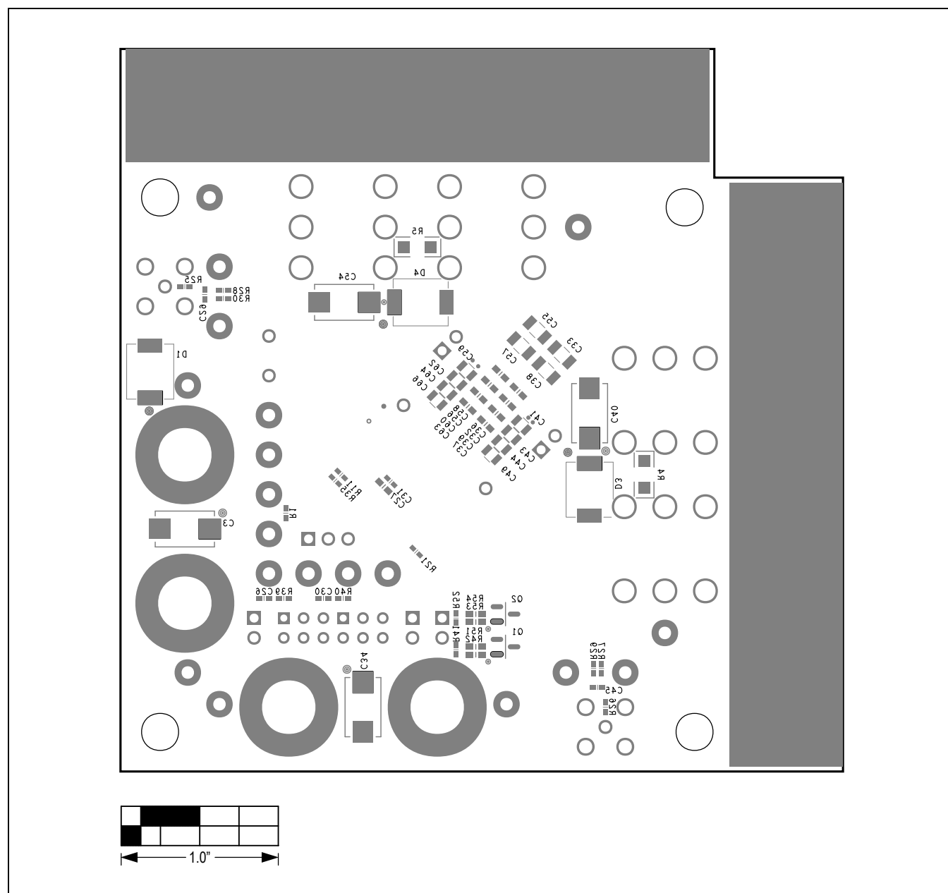
MAX20812 EV Kit PCB—Silkscreen Bottom Side
