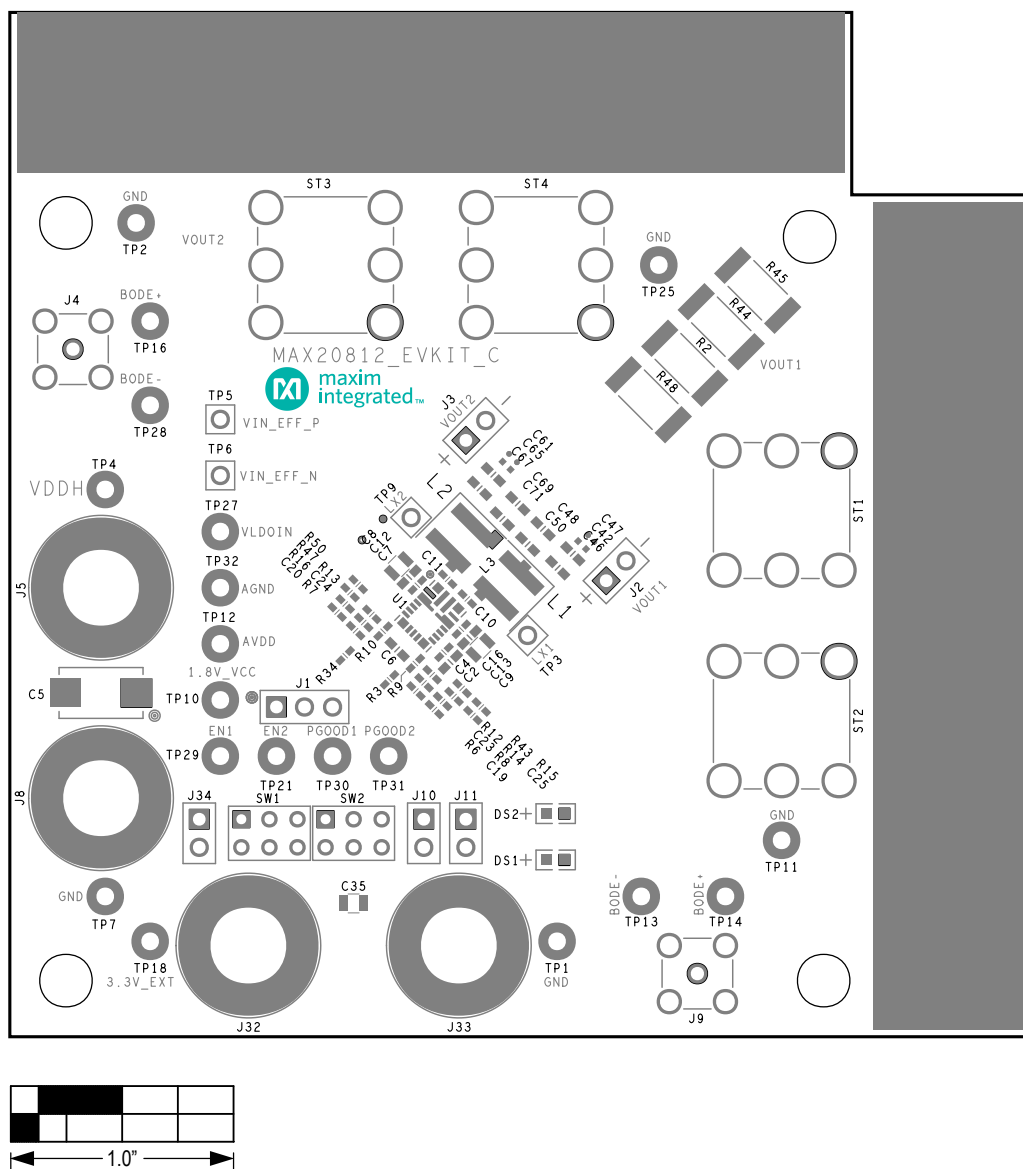
MAX20812 EV Kit PCB—Silkscreen Top Side
