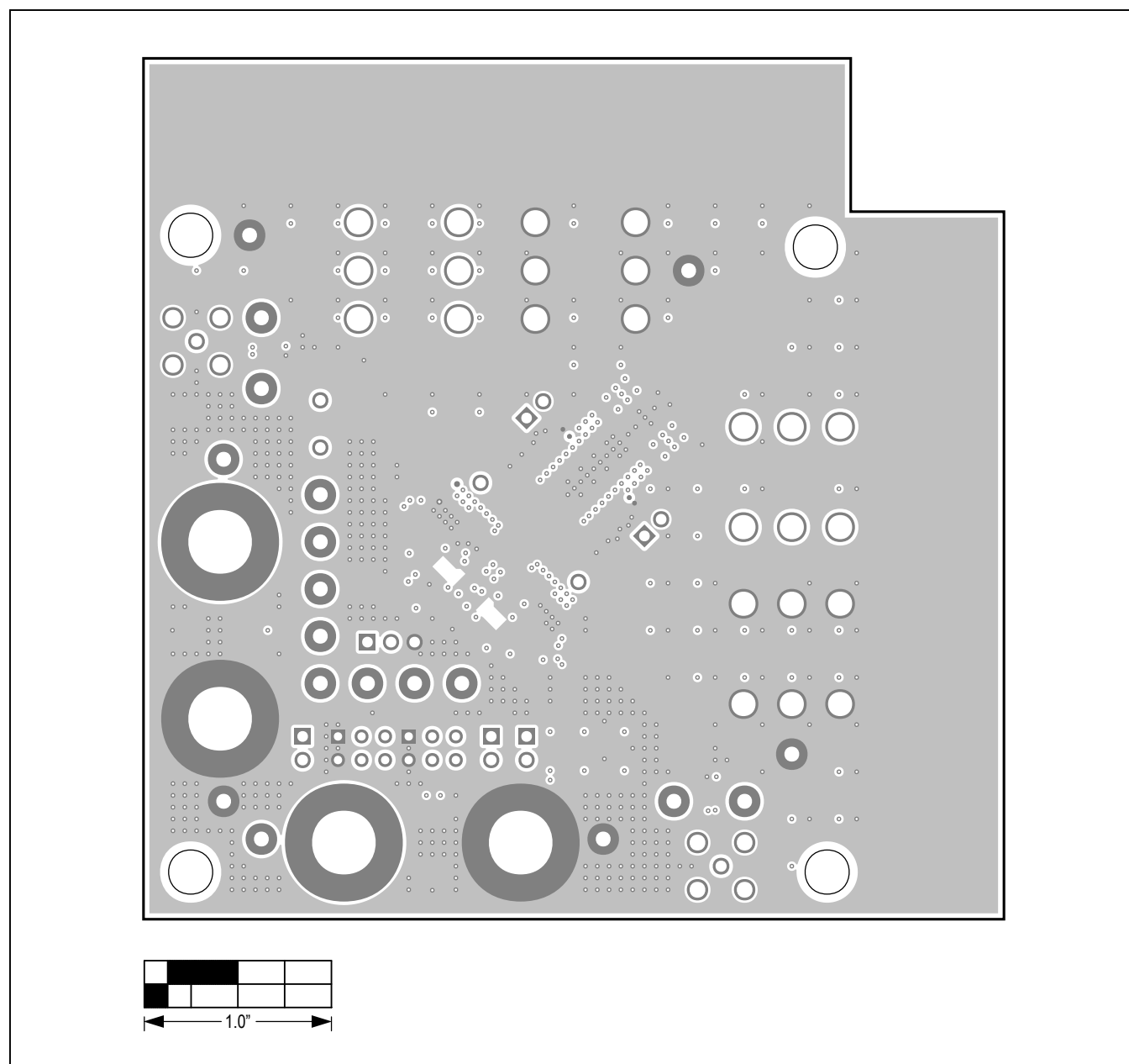
MAX20812 EV Kit PCB—Internal Layer 2
