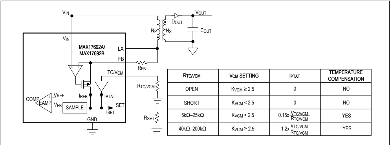
Figure 7. TC/VCML Pin Configuration
