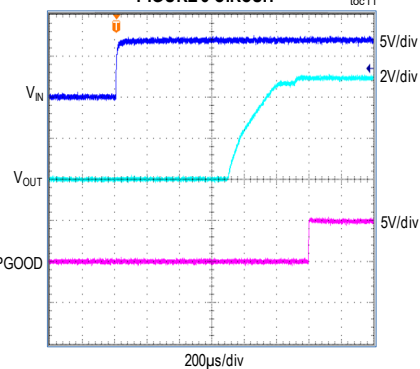
STARTUP RESPONSE WITH NO LOAD FIGURE 3 CIRCUIT
