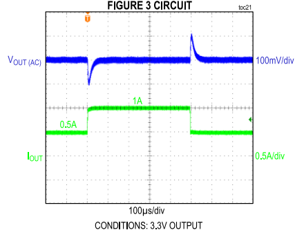
MAX17645B/MAX17645D LOAD TRANSIENT BETWEEN 0.5A AND 1A FIGURE 3 CIRCUIT
