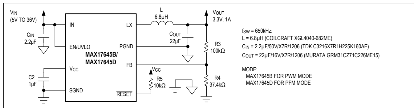
Figure 3. 3.3V, 1A Output Step-Down Regulator
