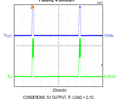
MAX17645B, OVERLOAD PROTECTION FIGURE 4 CIRCUIT
