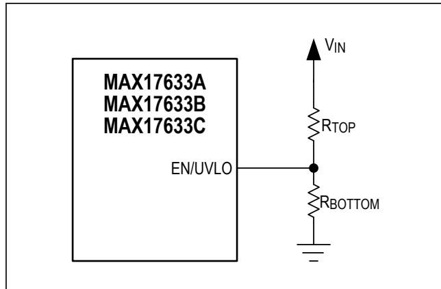
Figure 1. Setting the Input Undervoltage Lockout
