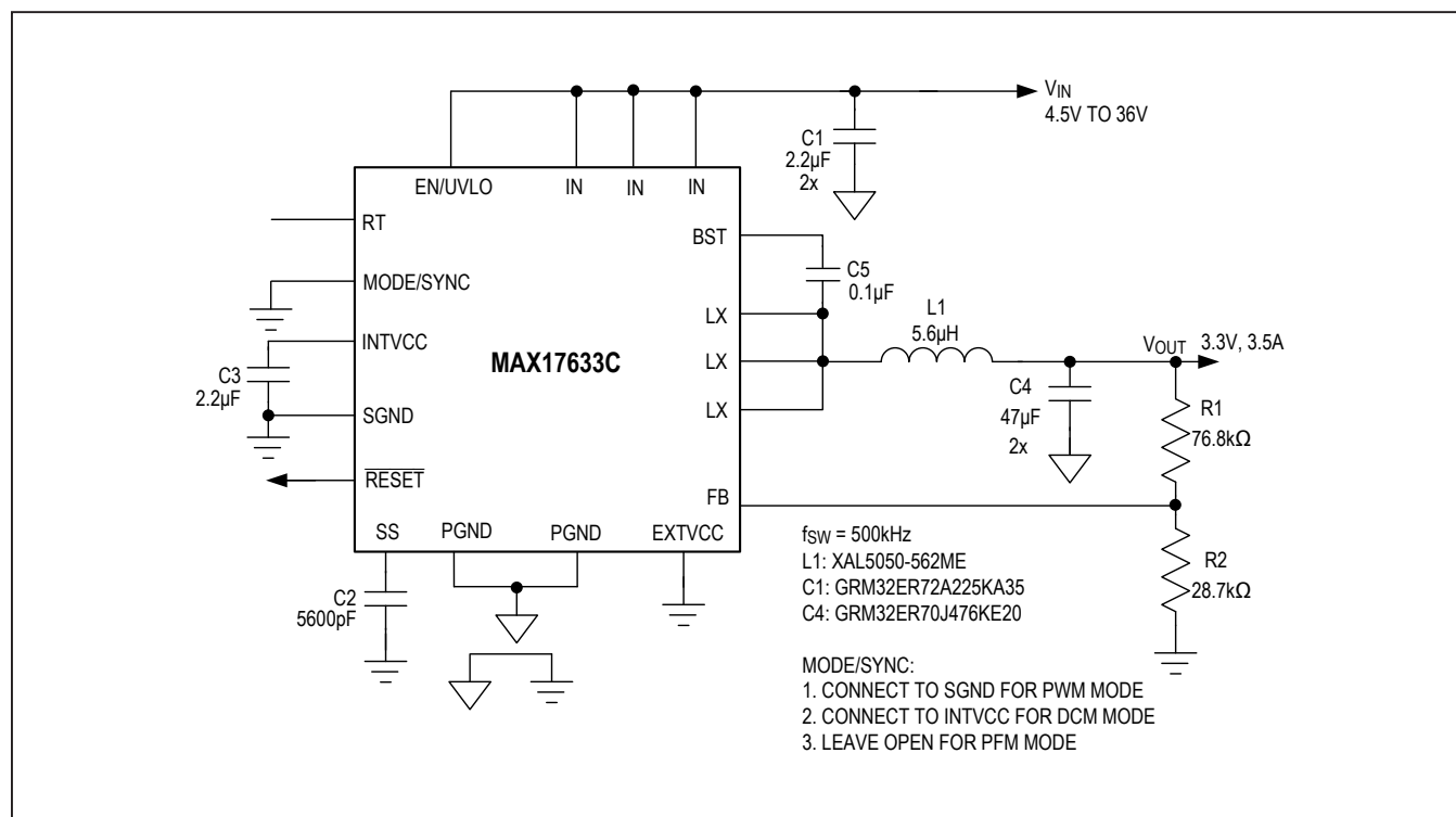
Figure 3. Adjustable 3.3V Output with 500kHz Switching Frequency
