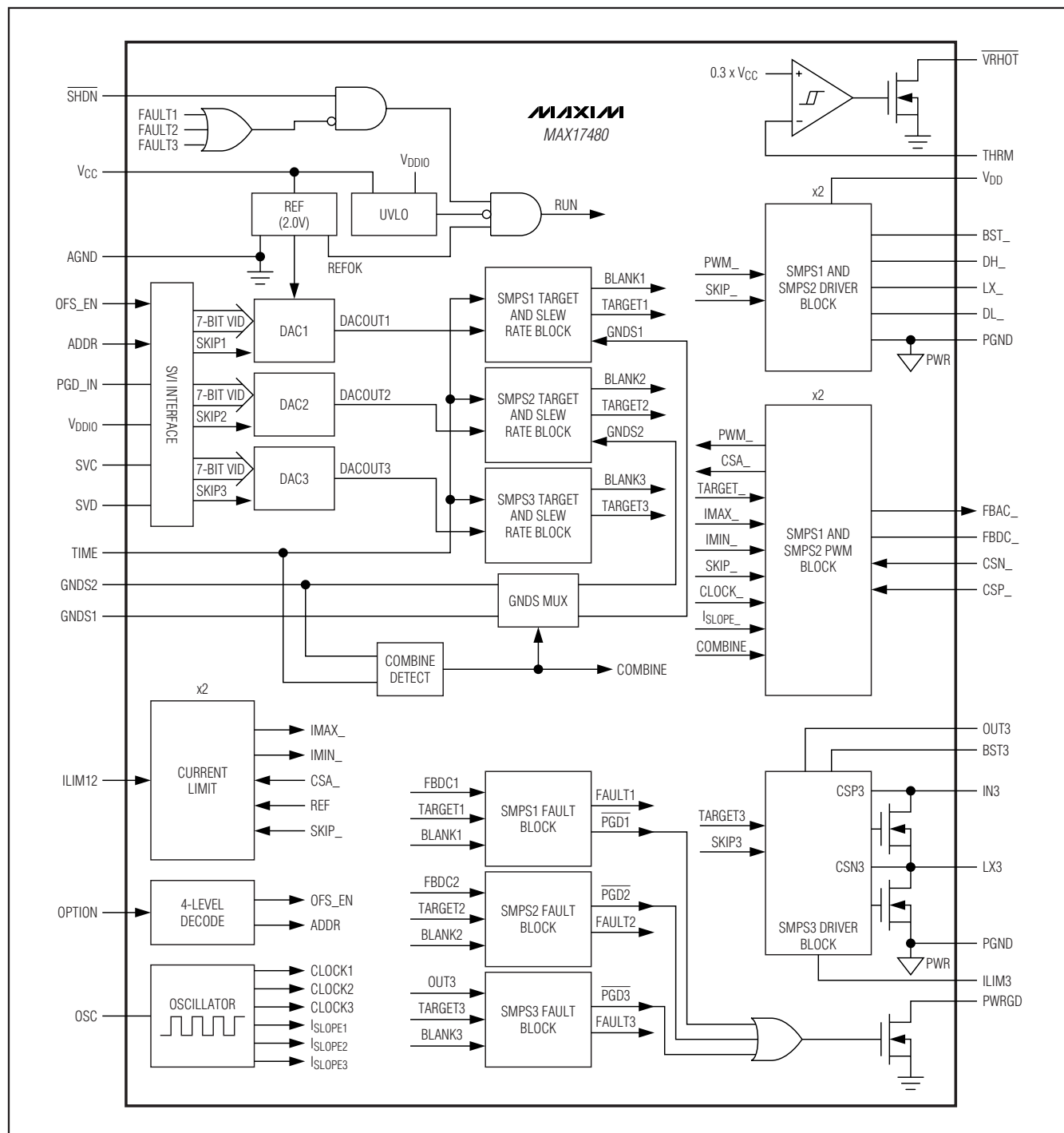
Figure 4. Functional Diagram
