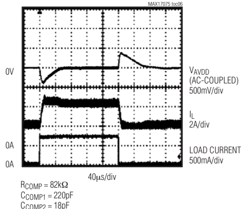
STEP-UP REGULATOR LOAD-TRANSIENT RESPONSE (100mA TO 800mA)
