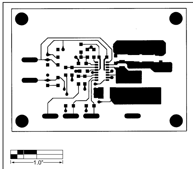
Figure 3. MAX1703 EV Kit PC Board Layout—Component Side
