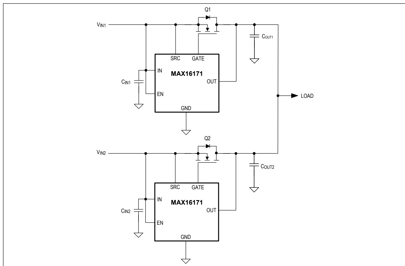
Figure 3. Redundant Power Supply Circuit
