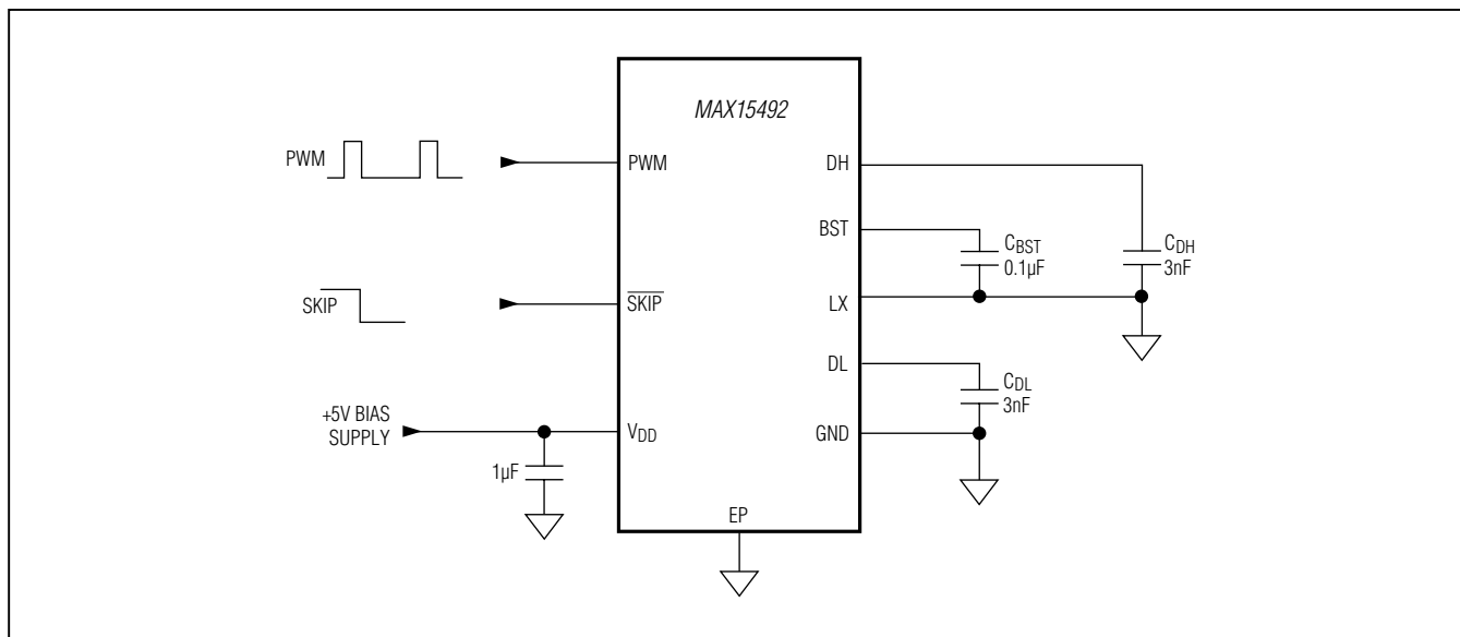
Figure 1. Test Circuit
