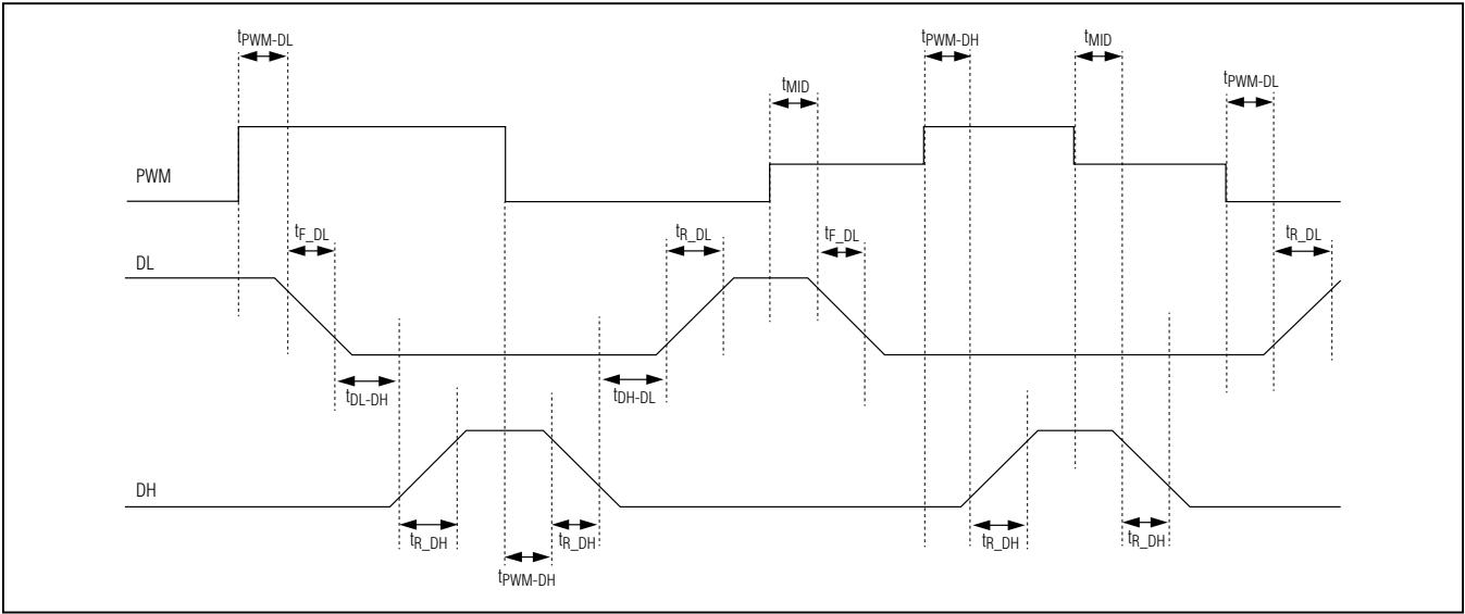
Figure 2. Timing Diagram
