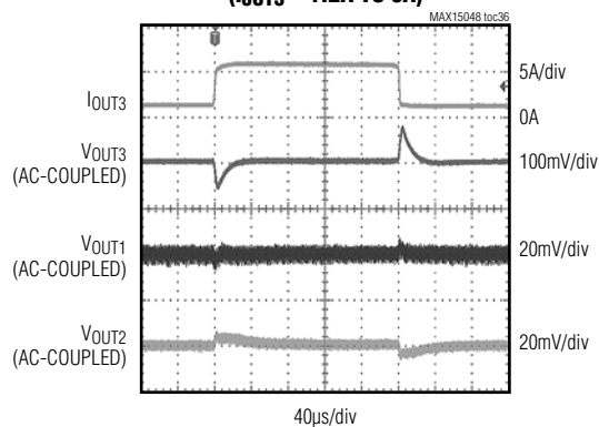
LOAD-TRANSIENT RESPONSE ( I_{OUT3} = 1.2A TO 6A )
