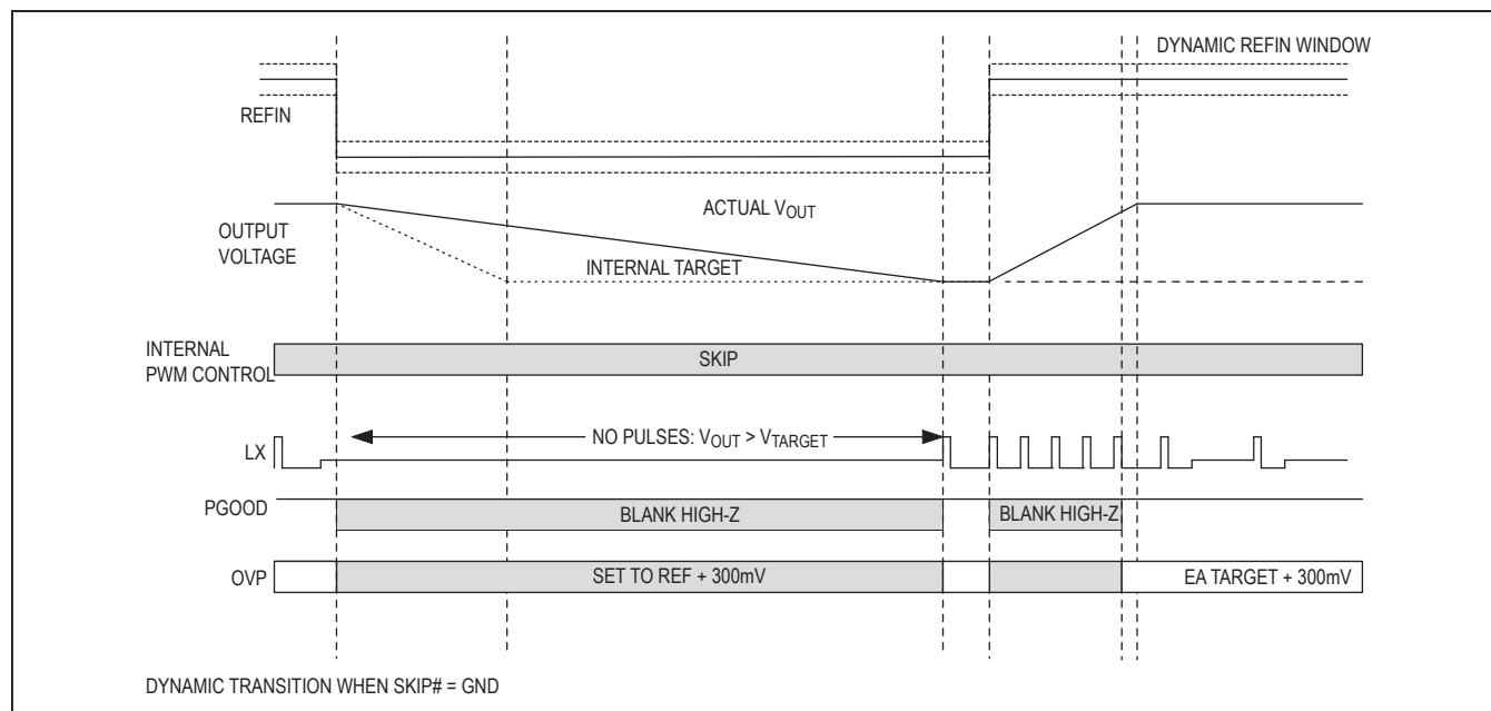
Figure 4. Dynamic Transition when \overline{\text{SKIP}} = \text{GND}
