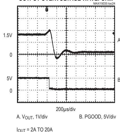
OUTPUT OVERVOLTAGE WAVEFORM
