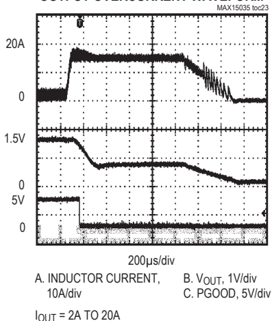
OUTPUT OVERCURRENT WAVEFORM
