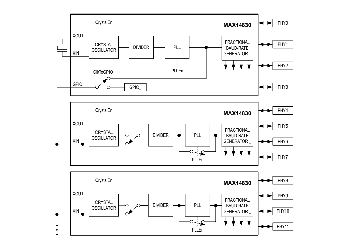
Figure 29. Interchip Synchronization
