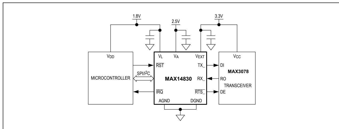
Figure 28. Logic-Level Translation
