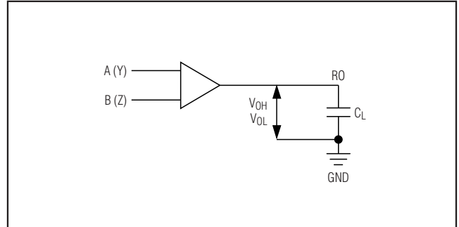
Figure 2. Receiver Differential Input
