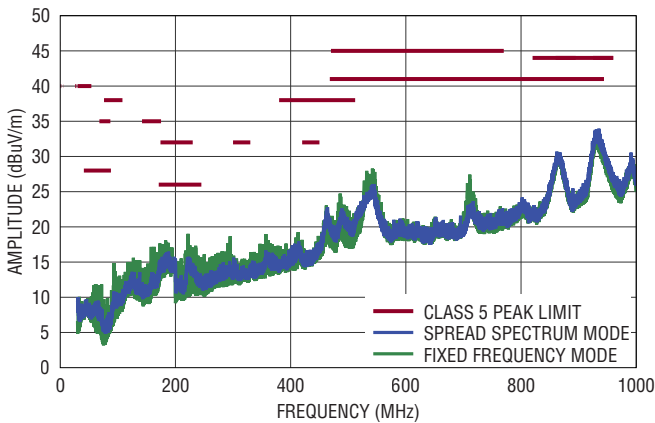
Radiated Peak
