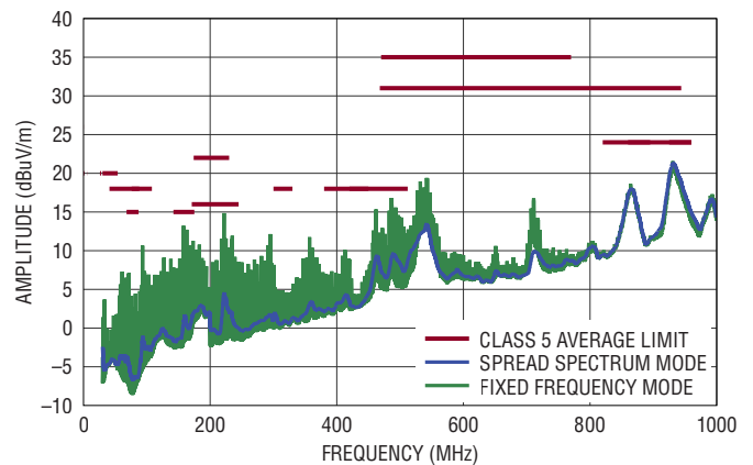
Radiated Average
