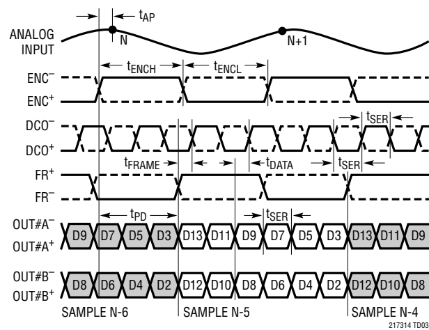
2-Lane Output Mode, 12-Bit Serialization
