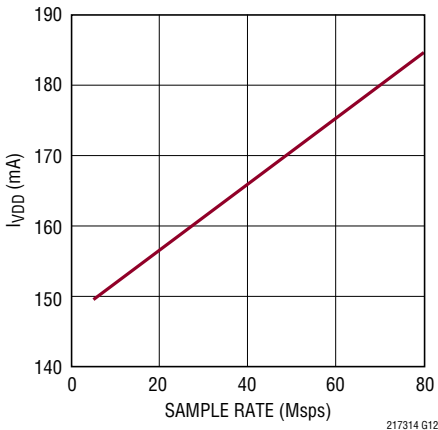
LTM2173-14: I_{VDD} vs Sample Rate, 5MHz Sine Wave Input, -1dBFS
