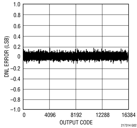
LTM2173-14: Differential Nonlinearity (DNL)
