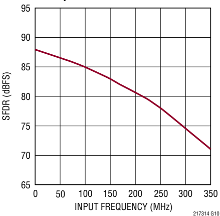
LTM2173-14: SFDR vs Input Frequency, -1dBFS, 2V Range, 80MSPS
