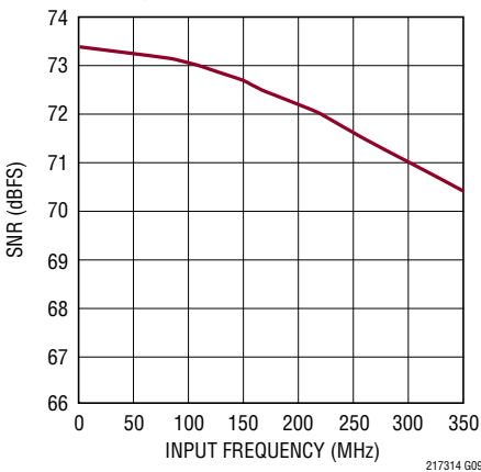
LTM2173-14: SNR vs Input Frequency, -1dBFS, 2V Range, 80MSPS
