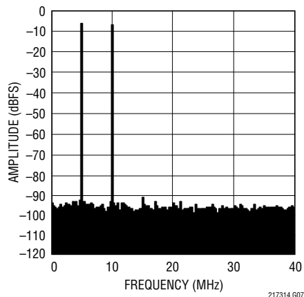
LTM2173-14: 8k Point 2-Tone FFT, f_{IN} = 70\text{MHz} , 75\text{MHz} , -7\text{dBFS} per Tone, 80Mps
