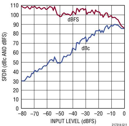
LTM2173-14: SFDR vs Input Level, f_{IN} = 70\text{MHz} , 2V Range, 80MSPS
