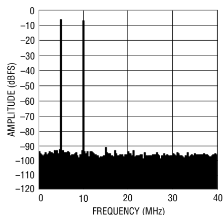
LTM2173-14, 80Msps, 2-Tone FFT, f_{\text{IN}} = 70\text{MHz} and 75\text{MHz}
