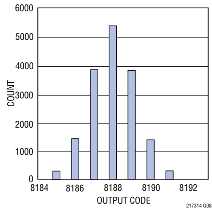
LTM2173-14: Shorted Input Histogram
