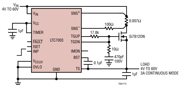
Figure 15. Design Example
