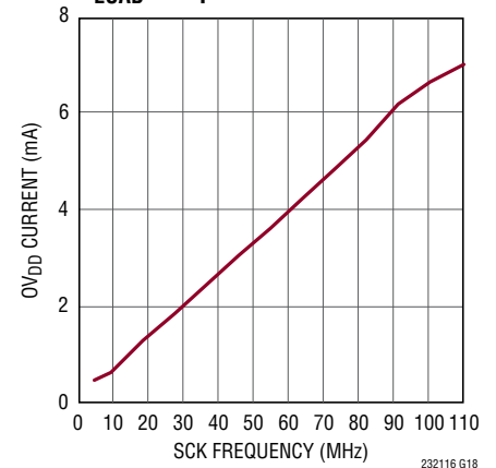
0V_{DD} Current vs SCK Frequency, C_{\text{LOAD}} = 10\text{pF}
