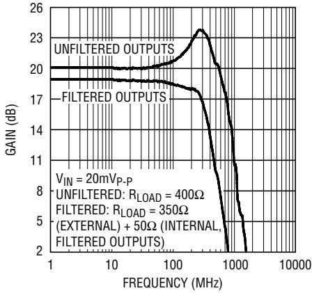
Frequency Response R LOAD = 400Ω
