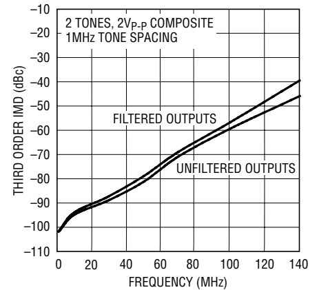
Third Order Intermodulation Distortion vs Frequency Differential Input, R LOAD = 100Ω
