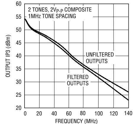
Output Third Order Intercept vs Frequency, Differential Input R LOAD = 100Ω
