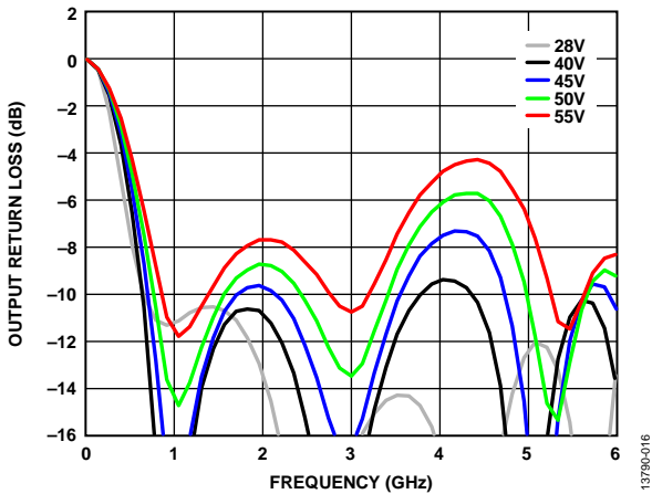
Figure 17. Output Return Loss vs. Frequency at Various Supply Voltages
